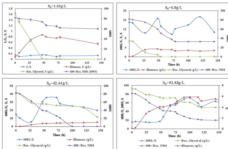
Fig. 1 Time course of total biomass in \text{g L}^{-1} ( X ), lipid in \text{g L}^{-1} ( L ) and residual glycerol in \text{g L}^{-1} ( S ), residual ammonium ion in \text{g L}^{-1} ( N ) for broth with initial glycerol concentration ( S_0 ) of 1.63 \text{ g L}^{-1} , 6.8 \text{ g L}^{-1} , 42.44 \text{ g L}^{-1} , and 92.83 \text{ g L}^{-1} .
