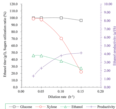
Fig. 3 Effect of dilution rate on ethanol production in continuous fermentation with cell recycling using S. stipitidis MA301.
