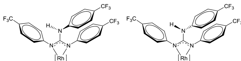
Fig. 2 Two rotamers of 2 . [Rh] = [( \eta^5 -Cp*)RhCl]. The two rotamers shown are distinct from each other when one considers the Cl as the reference atom.
