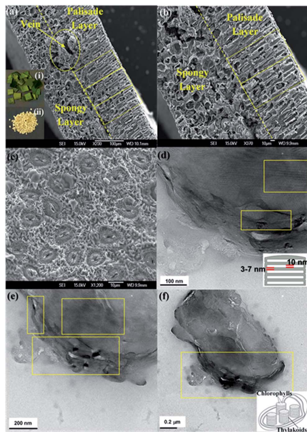
Fig. 2 (a and b) Cross-section SEM images of final catalysts, showing the well-replicated microarchitecture of the leaf photosystem. Inset: (i) photos of natural camellia sinensis leaves and (ii) TiO 2 artificial leaves. (c) Top-view SEM image of final catalysts, illustrating that the porous structure of the stomata is retained after the removal of the leaves. (d and e) TEM images of MNAL samples showing that the stack-layered nanostructures of the thylakoids in the chloroplast are retained after the removal of the leaves. (f) TEM images of AChl samples illustrating the well-replicated nano-architecture of the thylakoid membranes.
