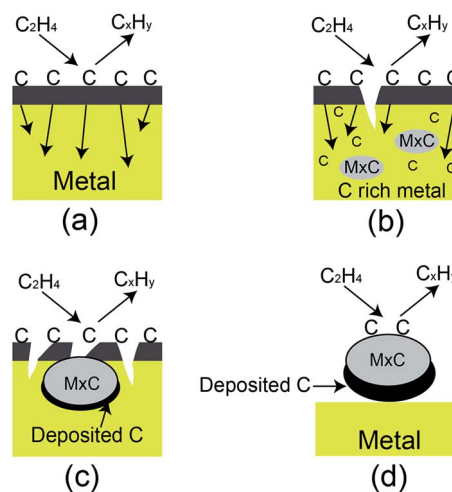
Fig. 2 The formation mechanism of carbon deposition onto the surface of stainless steel. Briefly, (a) \text{C}_2\text{H}_4 is adsorbed onto the surface of metal, (b) carbon atoms from \text{C}_2\text{H}_4 are diffused into the metal to form the metal carbides, (c) the formed metal carbides adsorb more carbon atoms from \text{C}_2\text{H}_4 , and (d) the carbon deposits grow.
