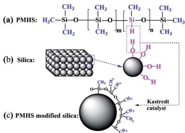
Fig. 2 Schematic representation of PMHS (a), silica (b) and PMHS modified silica (c).
