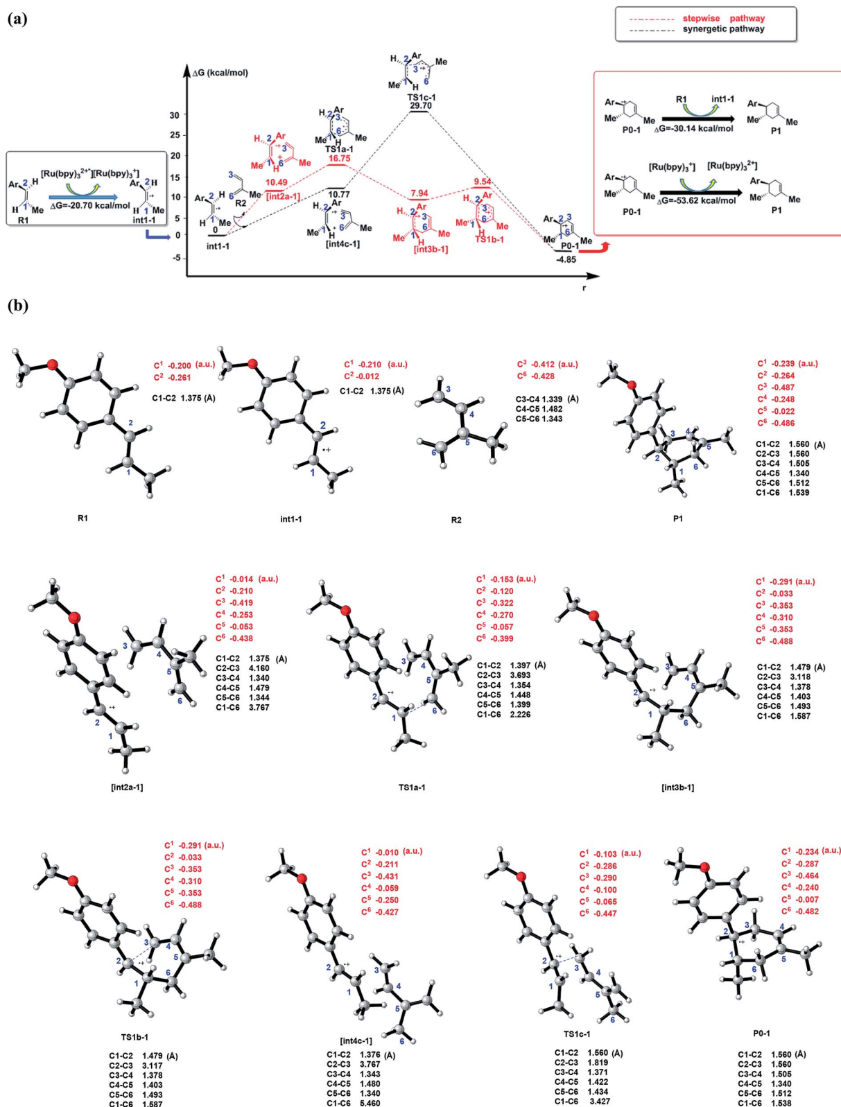
Fig. 2 (a) Schematic energy profiles of the C–C cycloaddition reaction between R1 + (dienophile) and R2 (diene). The red line is designed as the stepwise pathway and the black line is regarded as the synergetic pathway. The charge transformation to match the electronic properties is showed in the black box (start of cyclization) and red box (termination of the cyclization). [int2a-1] and [int4c-1] are the pre-reaction compounds after the molecular orientation in the corresponding pathways, which are stationary points on the potential energy surface. (b) The optimized structures, typical bond lengths (black) and NBO atomic charges (red) of all the stable states in (a) and transition states (by using CYLview 44 ).
