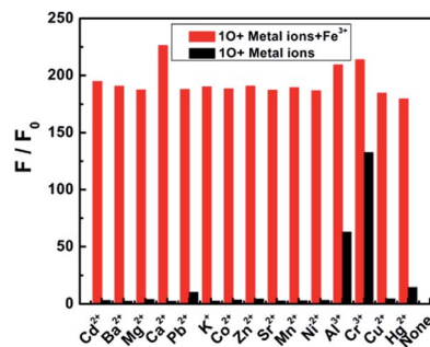
Fig. 5 Emission changes at 585 \text{ nm} of 10 in the presence of different metal ions added in the amount of 20.0 equiv. ( \lambda_{\text{ex}} = 515 \text{ nm} ) in acetonitrile/water binary solvent ( C = 2.0 \times 10^{-5} \text{ mol L}^{-1} , v/v = 1:1 ), after the initial addition of \text{Fe}^{3+} (10.0 equiv.) to the above solution.
