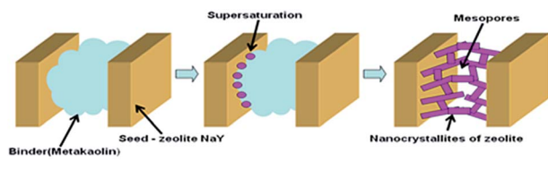
Fig. 5 The mechanism of formation of a hierarchical porous structure in meso-Y(60).
