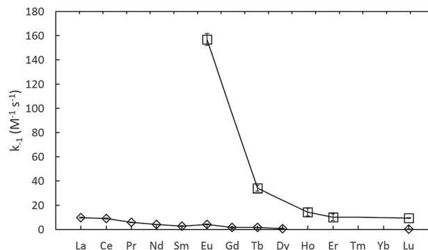
Fig. 5 Assumed decomplexation rate constants using arsenazo III, from Nash et al. 3 ( \diamond , in 0.3 M lactic acid) and using xylenol orange from this study ( \square , adjusted to 25 \text{ }^\circ\text{C} ).
