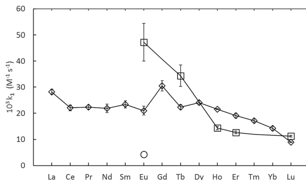
Fig. 4 Summary of measured lanthanide-dye-DTPA complexation kinetics from Shi et al. 26 (O, converted to second-order) Nash et al. 3 ( \diamond ) and this study ( \square , adjusted to 25 \text{ }^\circ\text{C} ). All data at pH 3.6.
