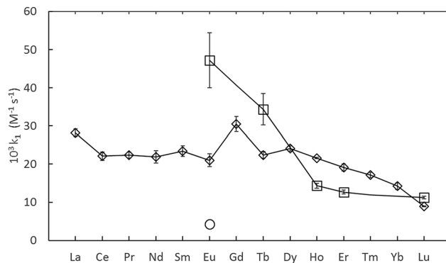
Fig. 4 Summary of measured lanthanide-dye-DTPA complexation kinetics from Shi et al. 26 (O, converted to second-order) Nash et al. 3 (◇) and this study (□, adjusted to 25 \text{ }^\circ\text{C} ). All data at pH 3.6.
