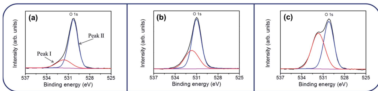
Fig. 5 XPS narrow scans of O 1s core level of various nanorod samples: (a) ZnO. (b) ZnO-SnO 2 . (c) ZnO-ZTO.
