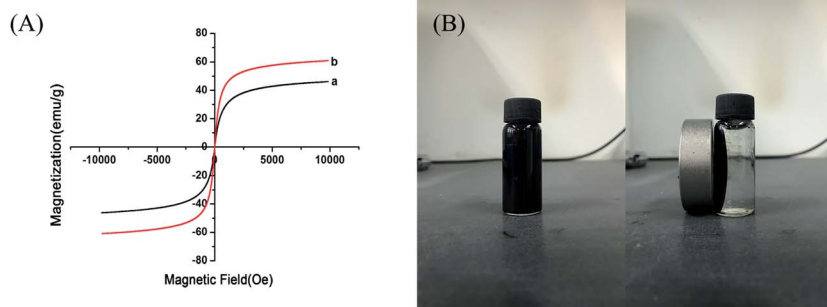
Fig. 2 (A) Magnetic hysteresis loops of GO@Fe 3 O 4 (a) and AMGO-Glu@Fe 3 O 4 (b), and (B) response of AMGO-Glu@Fe 3 O 4 to an external magnetic field.
