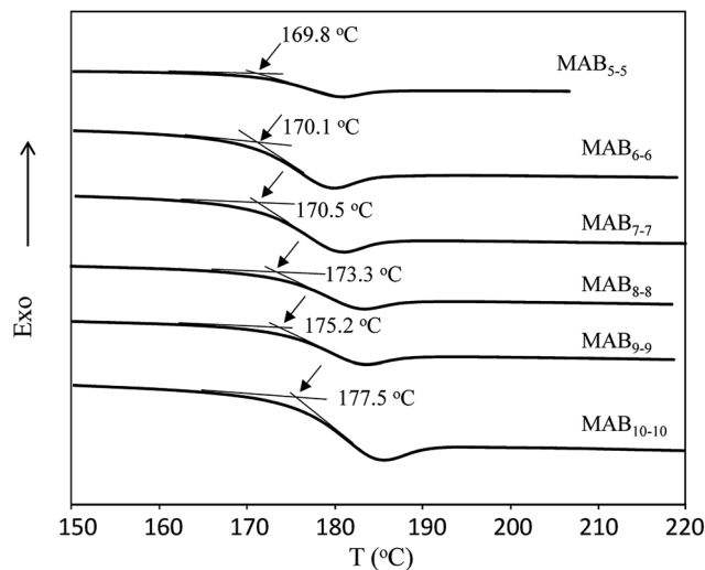
Fig. 4 DSC profiles of MAB x-x samples (heating rate 20 \text{ °C min}^{-1} , N 2 ).
