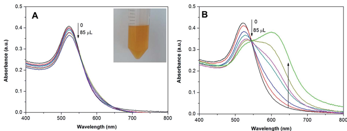
Fig. 7 UV-vis spectra of the \text{NaHSO}_4 -optimized AuNP sensor (2 mL) after the addition of 0, 10, 20, 40, 65, and 85 \mu\text{L} of the extracts from (A) blank human plasma (the inset is a photo of blank human plasma) and (B) berberine-containing human plasma (the extract contains 33.95 \mu\text{g mL}^{-1} berberine; final concentrations are 0, 0.24 \mu\text{g mL}^{-1}, 0.47 \mu\text{g mL}^{-1}, 0.91 \mu\text{g mL}^{-1}, 1.13 \mu\text{g mL}^{-1}, 1.45 \mu\text{g mL}^{-1}, and 1.86 \mu\text{g mL}^{-1} , respectively). The data were collected after 10 min.
