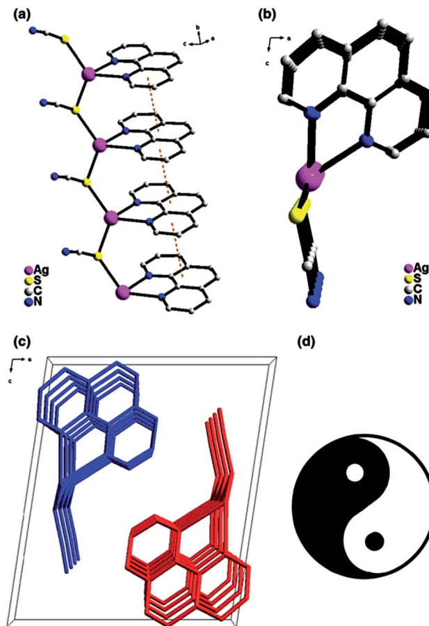
Fig. 17 (a) Diagram of the asymmetric chain in CP exhibiting strong \pi - \pi interactions among the phen rings (orange dash lines). (b) Perspective view of the chain along the b direction. (c) The unit cell packing structure of CP along the b direction. (d) The patterning of «Tai Ji». [Reprinted from ref. 204. Copyright 2016, with permission from Springer.]
