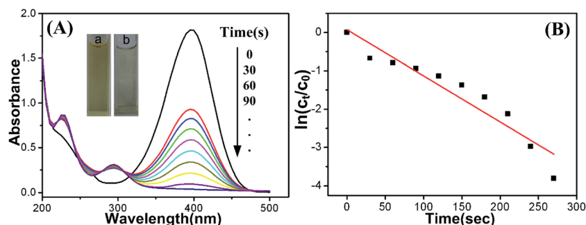
Fig. 5 (A) Time-dependent UV-vis spectral changes in p -nitrophenol solution catalyzed by Cu-doped CDs in the presence of \text{NaBH}_4 . Inset: the photograph of mixture containing p -nitrophenol and \text{NaBH}_4 before (a) and after (b) the addition of Cu-doped CDs under natural light. (B) Plots of \ln(C_t/C_0) versus time for the catalytic reduction of p -nitrophenol at room temperature.
