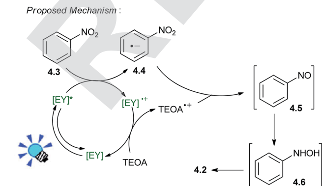
Scheme 4 Hydrogenation of nitroarenes to anilines.
