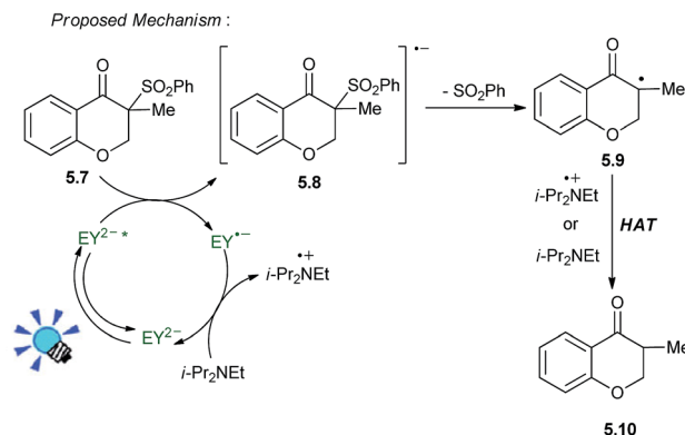
Scheme 5 Reductive desulfonylation of ketosulfones.
