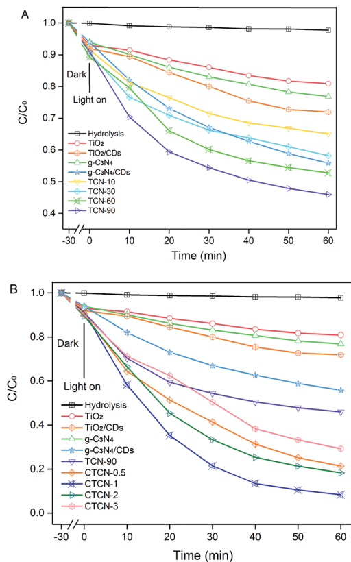
Fig. 9 Photocatalytic activity of \text{TiO}_2/g\text{-C}_3\text{N}_4 binaries (A) and \text{CDs}/\text{TiO}_2/g\text{-C}_3\text{N}_4 ternaries (B) based on the photocatalytic degradation of ENX under visible-light irradiation ( \lambda > 420 nm).
