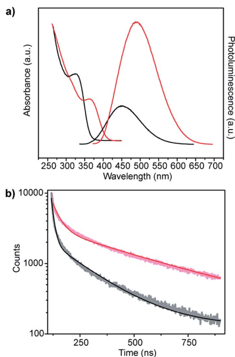
Fig. 6 (a) Absorption and corresponding photoluminescence spectra and (b) fluorescence decay-time measurements of \text{Zn}_{0.73}\text{Cd}_{0.27}\text{S} core-only (black) and \text{Zn}_{0.73}\text{Cd}_{0.27}\text{S} -ZnS (red) biomaterialized nanocrystals.
