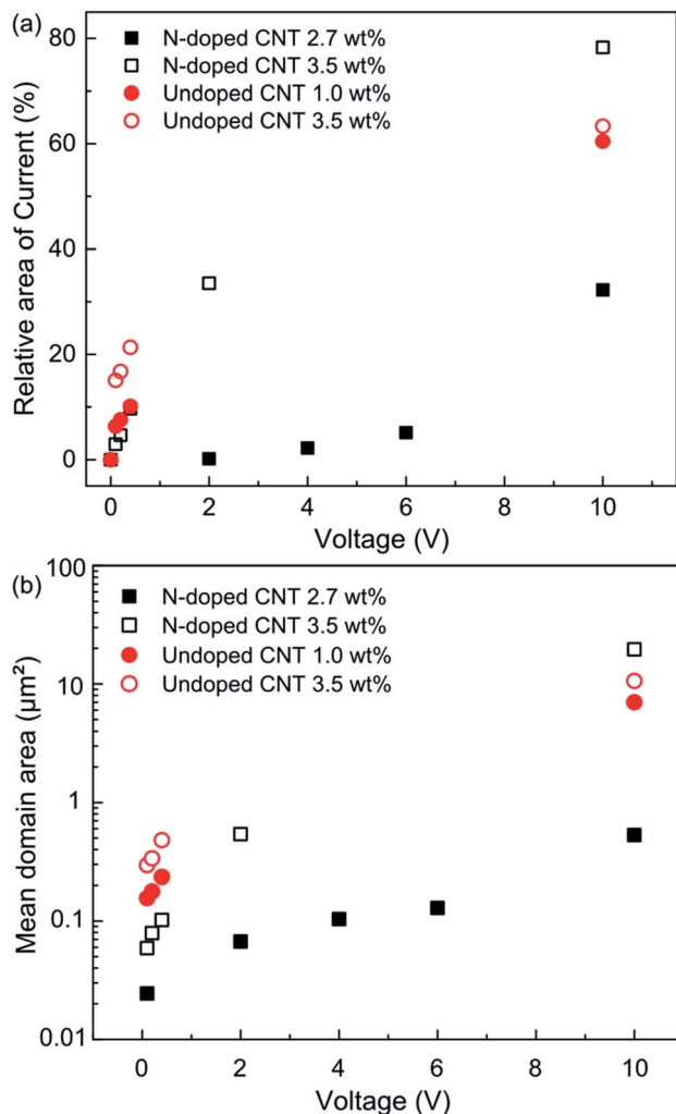
Fig. 10 (a) The percentage area (relative) of current observed per area scanned ( A_r ) and (b) the mean domain areas calculated for both N-doped (black filled/open squares) and undoped (red filled/open circles) CNT/PVDF nanocomposite samples. Filled squares/circles contain lower wt% CNTs, while open squares/circles contain 3.5 wt% CNTs.
