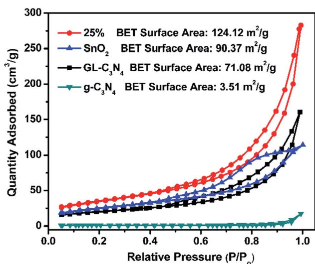
Fig. 4 N 2 adsorption-desorption isotherms of g-C 3 N 4 , GL-C 3 N 4 , SnO 2 and 25% SnO 2 /GL-C 3 N 4 composite.
