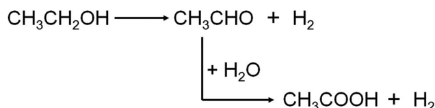
Scheme 2 Ethanol conversion to acetic acid via dehydrogenation–AWS reaction.
