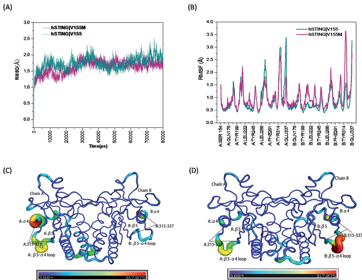
Fig. 2 The RMSD, RMSF and B -factor of hSTING in WT/MT systems. (A) The RMSD of backbone atoms (O, C, \alpha , N) in the MD simulations; (B) the RMSF of \alpha atoms during the last 50 ns of the MD simulations; (C) the B -factors ( \text{\AA}^2 ) of hSTING in wild type system during the last 50 ns of the MD simulation; (D) the B -factors ( \text{\AA}^2 ) of hSTING in V155M system (MT system) during the last 50 ns of the MD simulation.
