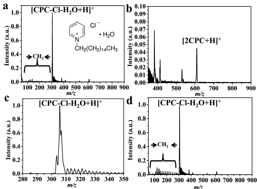
Fig. 5 SELDI-MS analysis of (a) CPC using CTS@Fe 3 O 4 MNPs; (b) magnification of the mass range of 350–900 Da, (c) the peak shape of the parent peak and (d) analysis of tap water.
