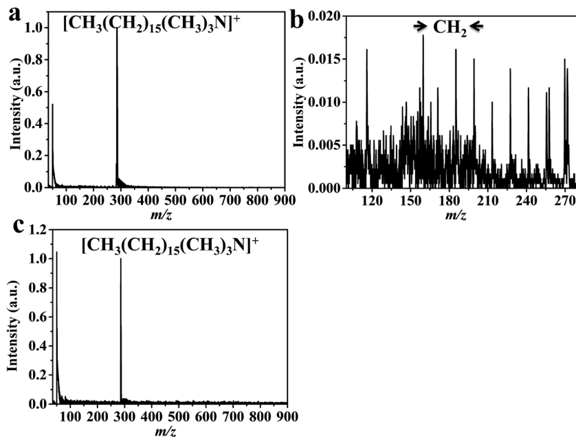
Fig. 4 SELDI-MS analysis of CTAB using CTS@Fe 3 O 4 MNPs; (a) from deionized water and (b) represent the magnification of the spectrum in the range of 100–280 Da, and (c) the analysis of tap water.
