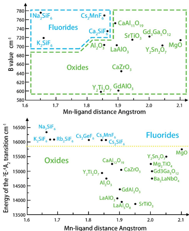
Fig. 4 Relationship between the Mn^{4+} ligand 21 bond distance and the Racah parameter B (top), and the position of the {}^2E_g level (bottom). 21
