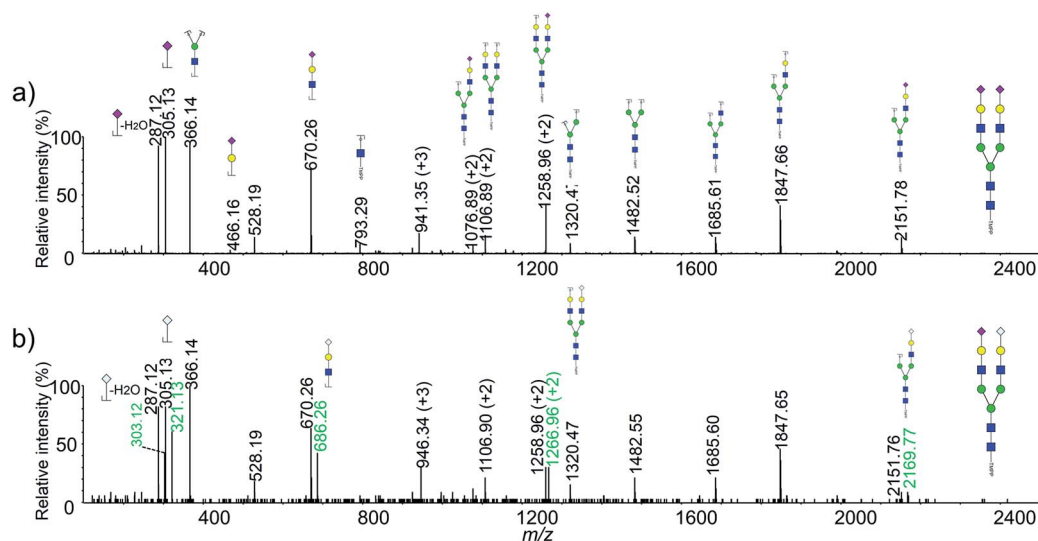
Fig. 3 Typical MS/MS spectra of the derivatized N-glycans from HeLa cell line. (a) NanoLC-ESI-MS/MS spectrum of m/z 941.35 [M + 3H]^{3+} with the composition of Hex 5 HexNAC 4 NeuAc 2 ; (b) NanoLC-ESI-MS/MS spectrum of m/z 946.34 [M + 3H]^{3+} with the composition Hex 5 HexNAC 4 NeuAc 1 NeuGc 1 .
