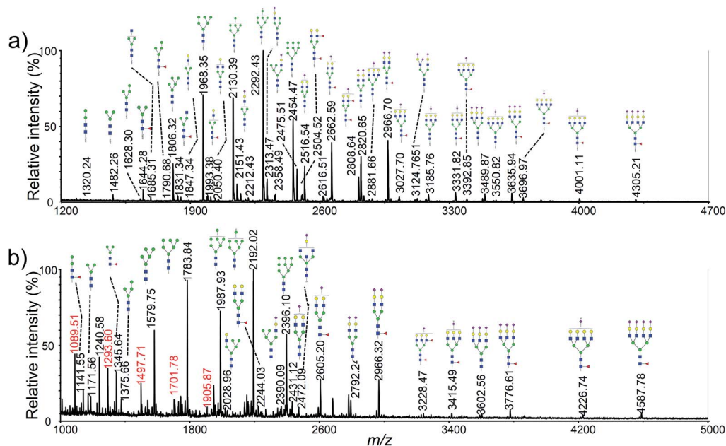
Fig. 2 Typical MALDI-TOF mass spectra of HeLa cell N-glycan profiling corresponding to 5 \times 10^5 cells with different sample preparations: (a) optimized method with co-derivatization; (b) traditional method with permethylation. Peaks with m/z values in red color in (b) correspond to polyhexose contaminations.
