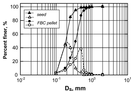
Fig. 5 Distributive and cumulative particle sizes of seed and FBC pellets (after 200 h operation of FBC under conditions of pH = 5.8 ± 0.2, [Fe(II)]/[P] = 1.75, U = 40.11 \text{ m h}^{-1} ).
