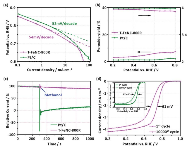
Fig. 5 (a) Tafel plots of T-FeNC-800R and Pt/C obtained from the RDE measurements. (b) H 2 O 2 yield and electron-transfer number ( n ) of T-FeNC-800R and Pt/C. (c) Current–time ( I – t ) curves of T-FeNC-800R and Pt/C in O 2 -saturated 0.1 M HClO 4 solution (without and with 1 M methanol). (d) LSV of T-FeNC-800R and Pt/C (inset) before and after 10 000 cycles in O 2 -saturated 0.1 M HClO 4 solution. All tests on a rotating disk electrode (900 rpm) with a scan rate of 10 mV s -1 .
