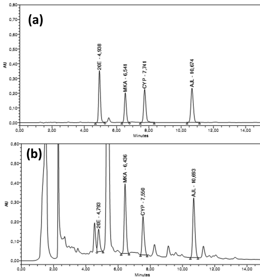
Fig. 3 HPLC chromatograms showing the elution of phytoecdysteroids. (a) Standard ecdysteroids ( 100 \text{ mg ml}^{-1} of each standard), (b) phytoecdysteroid elution pattern in one of the hairy root extract.
