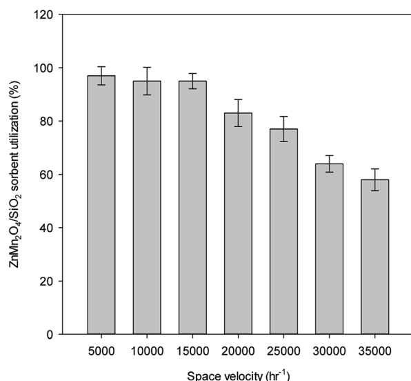
Fig. 4 Effect of space velocity on ZnMn 2 O 4 /SiO 2 sorbent utilization.
