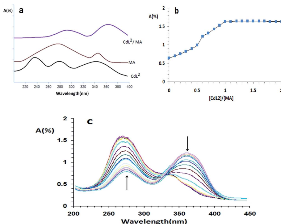
Fig. 1 A UV-Vis absorption spectra of solutions containing a concentration of CdL 2 ( 1.0 \times 10^{-3} mol L -1 ) and mafenamic acid (CdL 2 /MA), CdL 2 and mafenamic acid (MA) (a), plot of absorbance at 288 nm as function of mole ratio of [CdL 2 ]/[MA] (b) and electronic spectra of mole ratio of [CdL 2 ]/[MA] (c).
