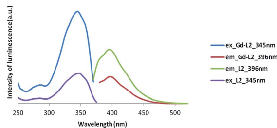
Fig. 6 Luminescence spectra of Gd complex of asymmetric ligand ( \text{Gd-L}^2 ) (excitation at 345 nm and emission at 396 nm).
