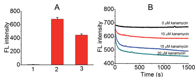
Fig. 2 ThT FL analysis for the kanamycin A induced FL displacement biosensor. (A) Depicts the ThT FL in different states. Column 1 = 1 \mu\text{M} ThT, 2 = 1 \mu\text{M} ThT + 1 \mu\text{M} KanaApt, and 3 = 2 + 20 \mu\text{M} kanamycin A. (B) Shows the real-time fluorescence when different concentrations of kanamycin A (0 to 20 \mu\text{M} ) were added to the 1 \mu\text{M} KanaApt–ThT complex.
