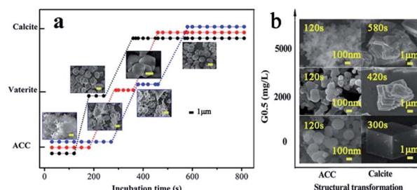
Fig. 2 (a) Schematic diagram of the CaCO 3 structural transformation from ACC to calcite via vaterite with different concentrations of G0.5 (● control, (●) 2000 mg L -1 and (●) 5000 mg L -1 ) the colour of the spherules should be black (control), red (2000 mg L -1 ) and blue (5000 mg L -1 ), respectively versus incubation time, which was obtained with a combination analysis of the pXRD, FTIR and SEM results and (b) schematic diagram of the CaCO 3 structural transformation by SEM.
