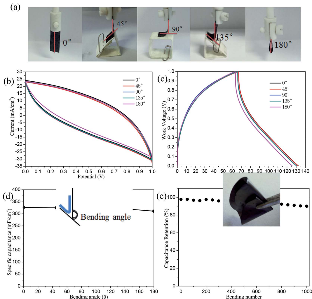
Fig. 7 (a) Photographs of the films bended to different angles; (b) CV and (c) GCD curves of the electrodes at different bending angle of 0^\circ , 45^\circ , 90^\circ , 135^\circ , and 180^\circ ; (d) specific capacitance at different bending angles; (e) efficiency of the films after different bending cycles at the current density of 5 \text{ mA cm}^{-2} .
