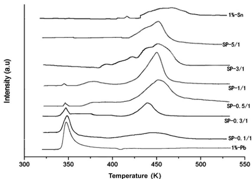
Fig. 5 The TPR profiles of the catalysts.
