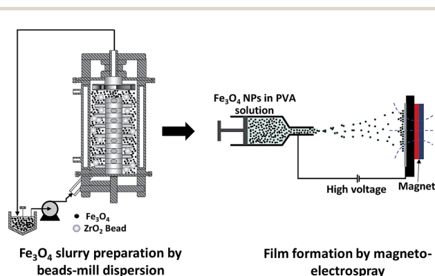
Fig. 1 Schematic illustration of the preparation process of Fe 3 O 4 nanoparticle films.
