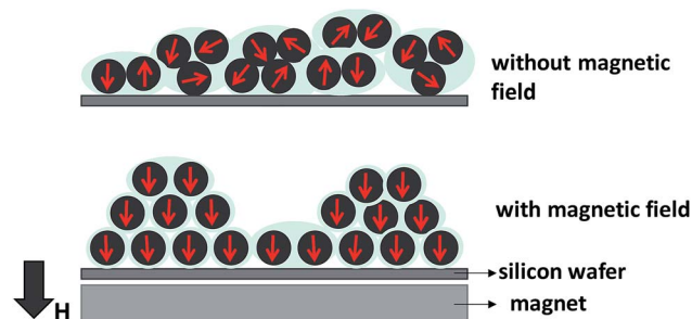
Fig. 9 Illustration of the magnetic nanoparticle direction inside films deposited with and without a magnetic field.
