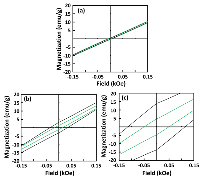
Fig. 4 Hysteresis loops of 10 (a), 25 (b), and 45 nm (c) \text{Fe}_3\text{O}_4 nanoparticles. Black and green lines correspond to before and after dispersion, respectively.
