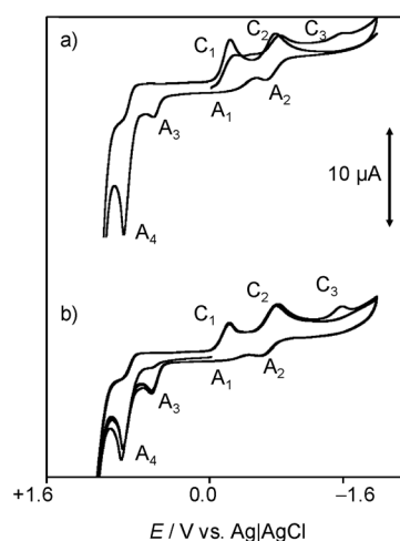
Fig. 2 Cyclic voltammograms at glassy carbon electrode of a 0.03 mM chartreusin solution in 0.10 M \text{Bu}_4\text{NPF}_6/\text{DMSO} (1% water v/v). (a) Initial cathodic scan; (b) initial anodic scan. Potential scan rate 50 \text{ mV s}^{-1} .
