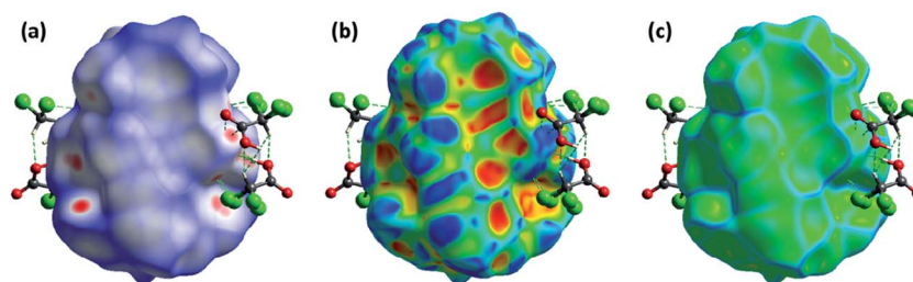
Fig. 3 Hirshfeld surface mapped with d_{\text{norm}} (left), shape index (middle), and curvedness (right) for the title cocystal [Cu 2 (valdien) 2 ]·2Cl 2 -CHCOOH 1.
