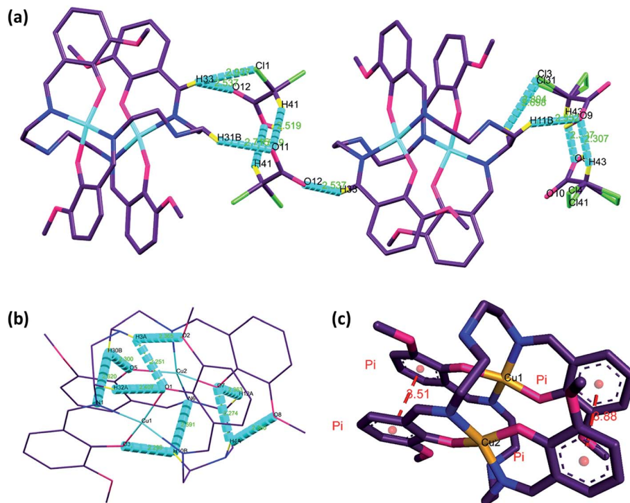
Fig. 2 Non-covalent interaction of cocystal [Cu 2 (valdien) 2 ]·2Cl 2 CHCOOH 1. (a) Inter-molecular C–H...O and C–H...Cl hydrogen bonding interaction. (b) C–H...N, C–H...O, and N–H...O, intra-molecular hydrogen bonding interaction. (c) π...π stacking interactions.
