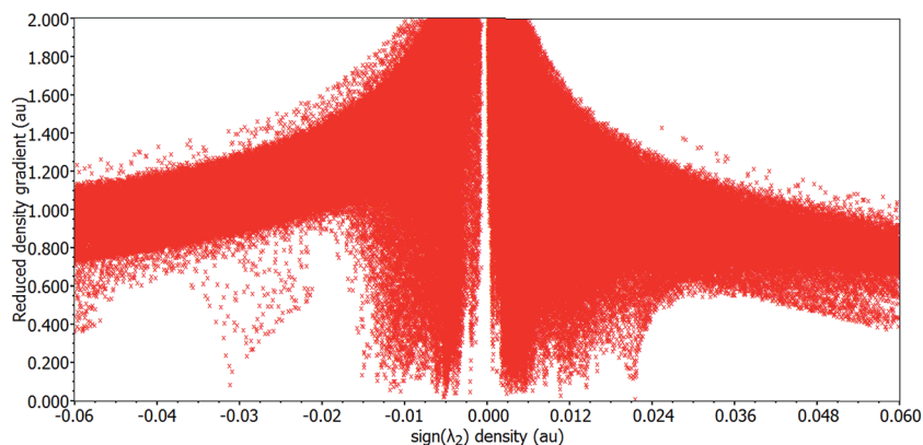
Fig. 5 Plot of the reduced density gradient versus the electronic density multiplied by the sign of the second Hessian eigenvalue of cocrystal [\text{Cu}_2(\text{valdien})_2] \cdot 2\text{Cl}_2\text{CHCOOH} 1 .
