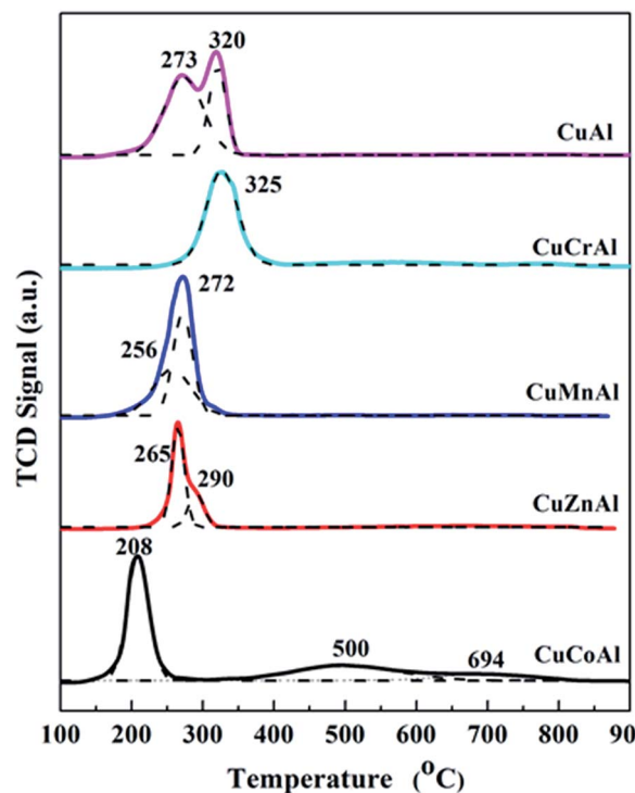
Fig. 2 TPR profiles of the calcined CuMAl samples.
