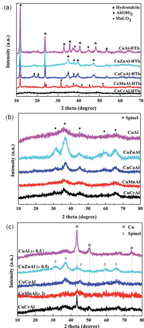
Fig. 1 XRD patterns of Cu, M, Al-LDHs (a), after calcination (b) and after reduction (c).
