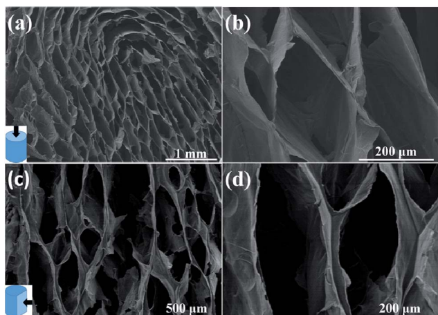
Fig. 2 SEM images of (a, b) cross-section and (c, d) vertical-section of the graphene aerogel.
