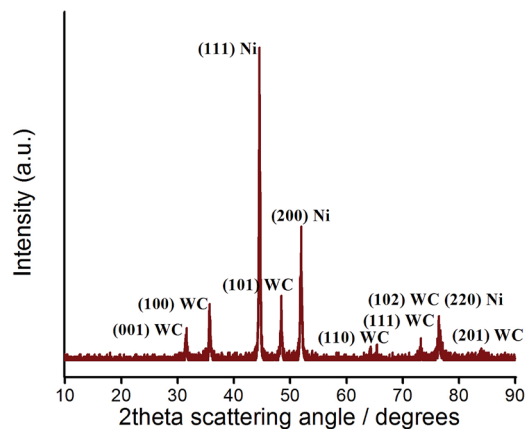
Fig. 8 XRD pattern of as-prepared coating by 6 \text{ A dm}^{-2} , 20 \text{ g dm}^{-3} , 400 \text{ rpm} .
