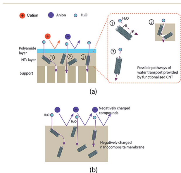
Fig. 8 Mechanism of functionalized CNT (mixed-matrix) in improving membrane performance. (a) Possible pathways of water transport provided by functionalized CNT and (b) rejection of negatively charged compounds.
