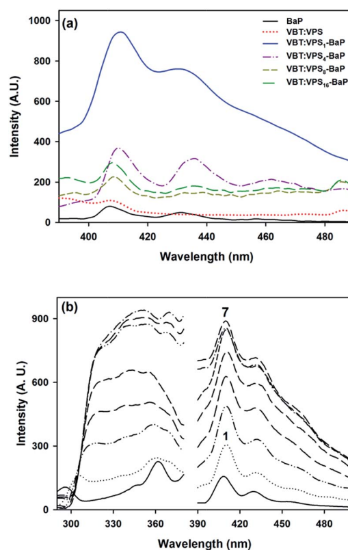
Fig. 3 (a) Fluorescence emission spectra of aqueous solutions of BaP ( 5 \times 10^{-3} mg L -1 ) and VBT : VPS m copolymers ( 5 \times 10^3 mg L -1 ), with m = 1, 4, 8 and 16 ( \lambda_{\text{exc}} = 300 nm). (b) Fluorescence emission and excitation spectra of seven water solutions of VBT : VPS 1 and BaP ( \lambda_{\text{ems}} = 410 nm, \lambda_{\text{exc}} = 360 nm). VBT : VPS 1 concentration was varied from 0.5 \times 10^3 mg L -1 (line labelled “1”) to 6.5 \times 10^3 mg L -1 (line labelled “7”), in steps of 1 \times 10^3 mg L -1 , while the BaP concentration was set to 5 \times 10^{-3} mg L -1 . Fluorescence spectrum of a BaP solution at 5 \times 10^{-3} mg L -1 is shown in solid line.
