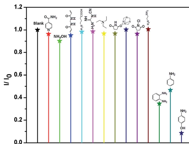
Fig. 4 Room-temperature luminescent intensity of Eu-MOF at 613 nm in MeOH suspension of Eu-MOF with 110 ppm of different organic amines ( \lambda_{\text{ex}} = 317 nm).
