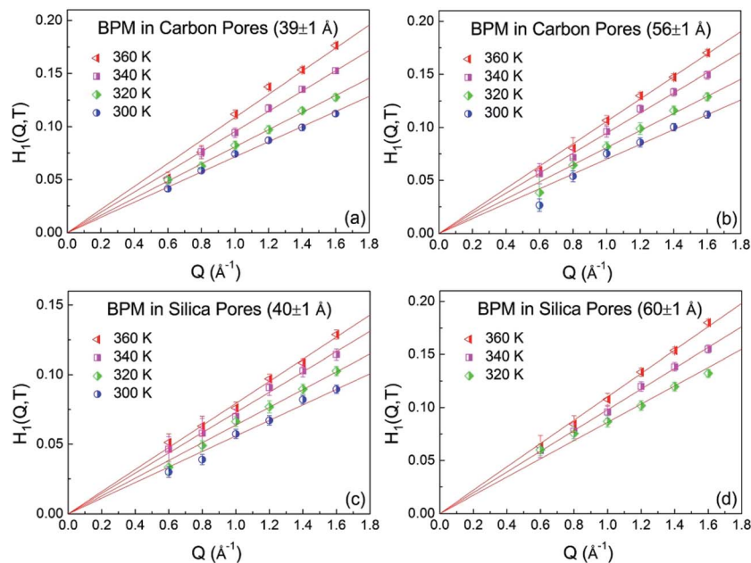
Fig. 4 Q dependence of fitting parameter H_1(Q,T) for BPM confined in carbon pores ( 39 \text{ \AA} ) (a), carbon pores ( 56 \pm 1 \text{ \AA} ) (b), silica pores ( 40 \pm 1 \text{ \AA} ) (c) and silica pores ( 60 \pm 1 \text{ \AA} ) (d) at different temperatures.
