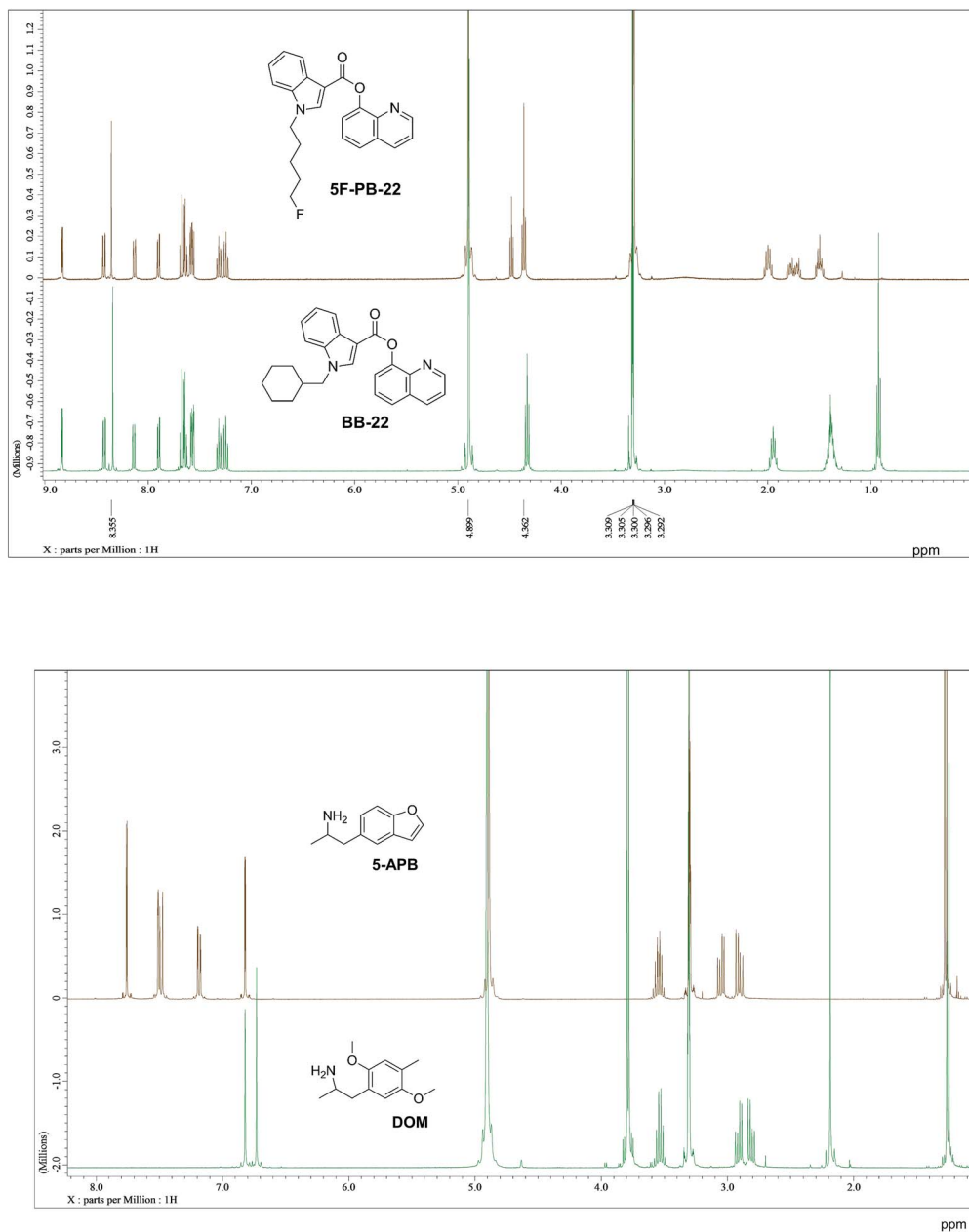
Fig. 7 1\text{D } ^1\text{H} NMR spectra of representative NPS (green) and the members of their respective clusters (brown). Full spectral range for 5-APB and DOM available in ESI.†
