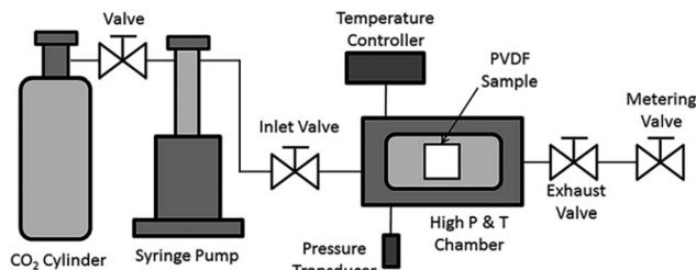
Fig. 1 Schematic illustration of a batch foaming system.
