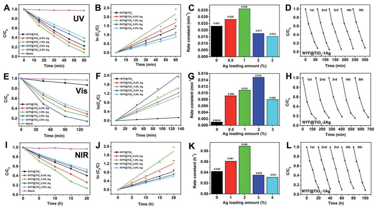
Fig. 3 Photocatalytic degradation of MO aqueous solution in the present of the \text{NYF@TiO}_2-x wt% Ag ( x = 0, 0.5, 1, 2, and 3 ) photocatalysts under (A–D) UV, (E–H) visible (I–L) NIR light irradiation. The plot of (C/C_0) vs. reaction time (A, E, I), \ln(C_0/C) vs. reaction time (B, F, J), the apparent rate constants vs. Ag loading (C, G, K), photocatalytic stability in five successive cycling reactions (D, H, L).
