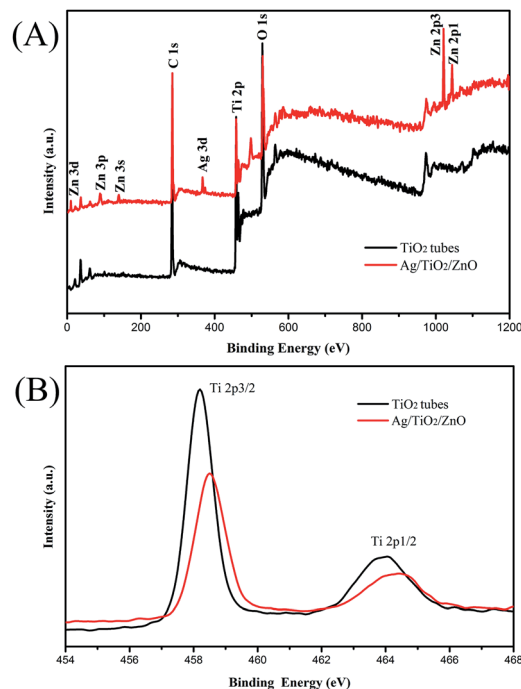
Fig. 4 The XPS spectra of the TiO 2 and ATZ nanotubes: (A) full spectrum of the sample and (B) the Ti 2p spectrum.
