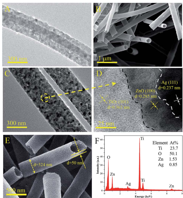
Fig. 3 The TEM image of the TiO 2 nanotubes (A). SEM image of the ATZ nanotubes (B). The TEM image of the ATZ nanotubes (C) and the HRTEM of the ATZ nanotubes (D). A high magnification SEM image of a ATZ nanotube (E) and the EDX spectra of the ATZ nanotubes (F).
